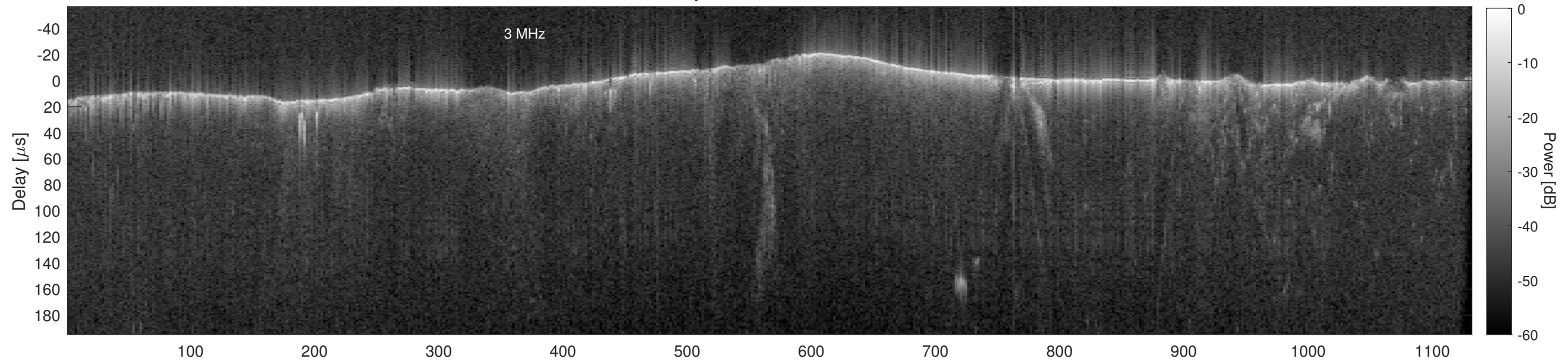
Orbit 21789, Cluttergram
