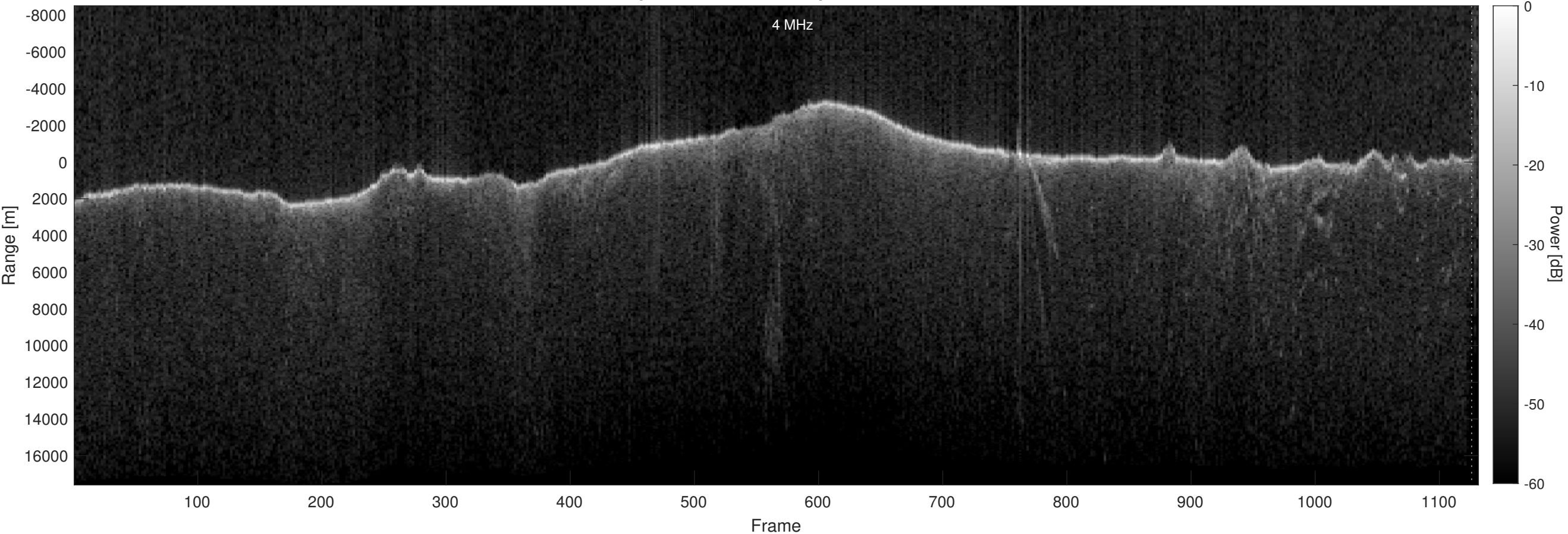
Orbit 21789, Optimized, Window, Depth-Corrected, Channel 2
