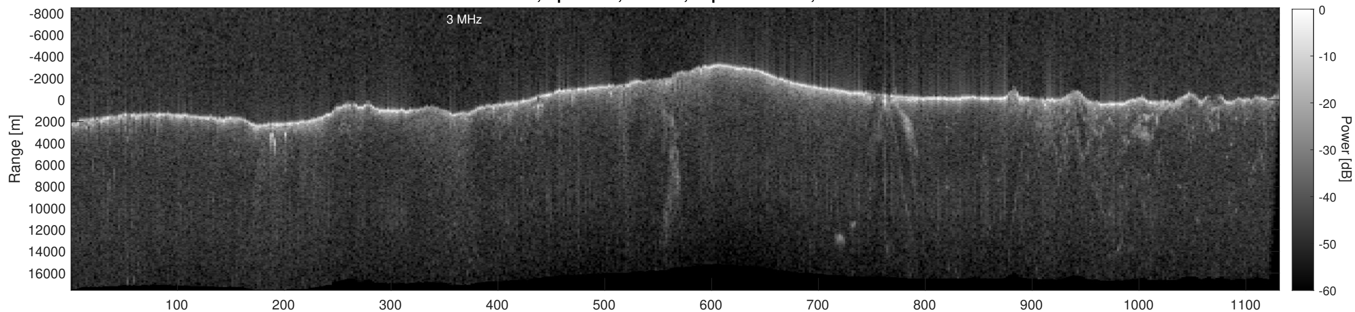
Orbit 21789, Depth-Corrected Cluttergram
