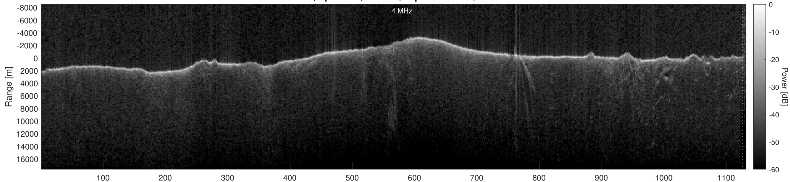
Orbit 21789, Optimized, Window, Depth-Corrected, Channel 2
