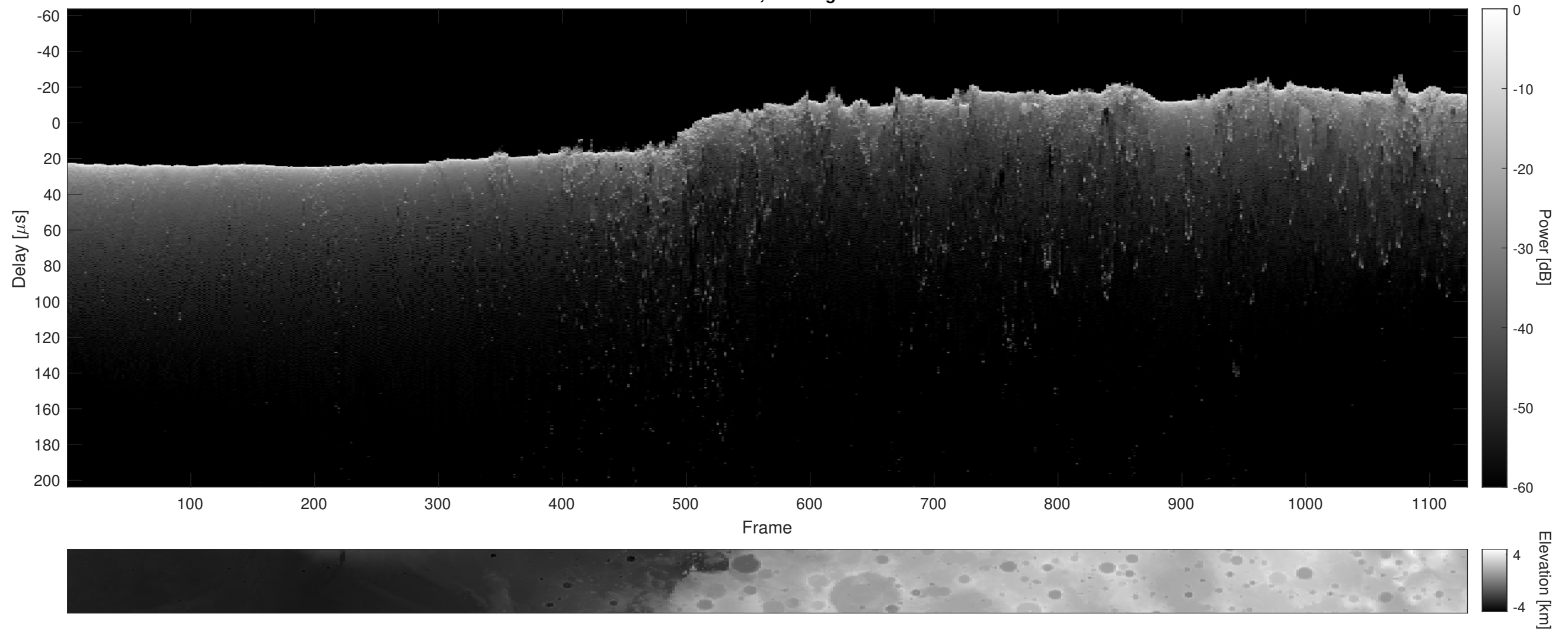
Orbit 21790, Cluttergram
