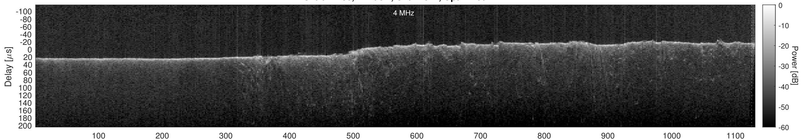
Orbit 21790, Cluttergram
