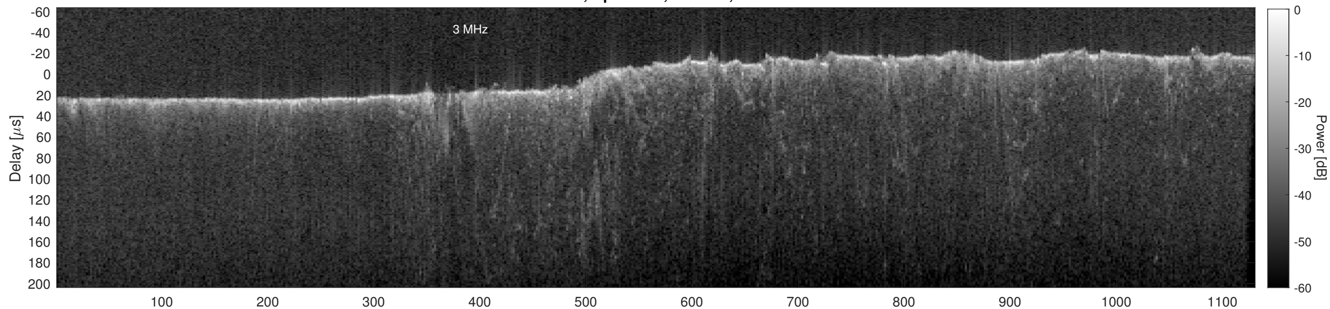
Orbit 21790, Cluttergram
