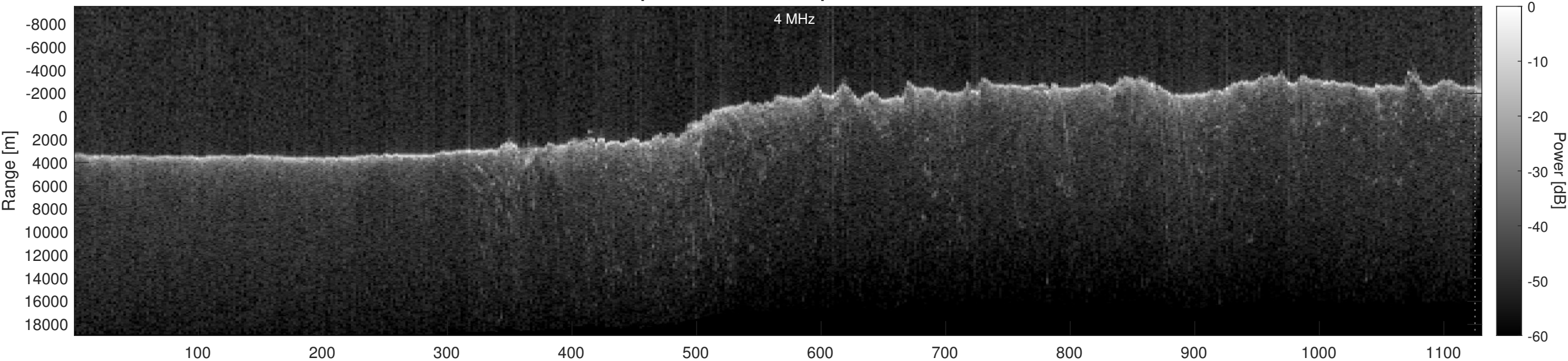
Orbit 21790, Optimized, Window, Depth-Corrected, Channel 2
