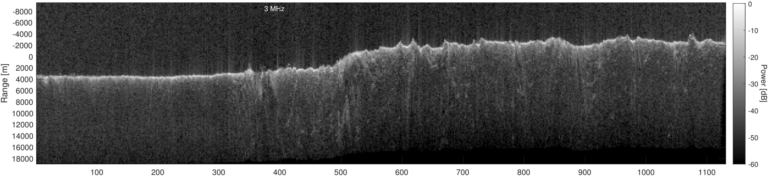
Orbit 21790, Depth-Corrected Cluttergram
