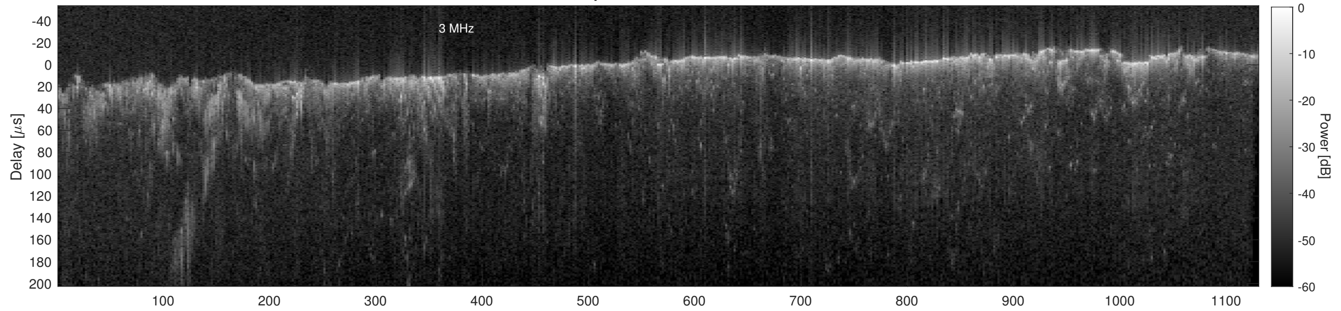
Orbit 21791, Cluttergram
