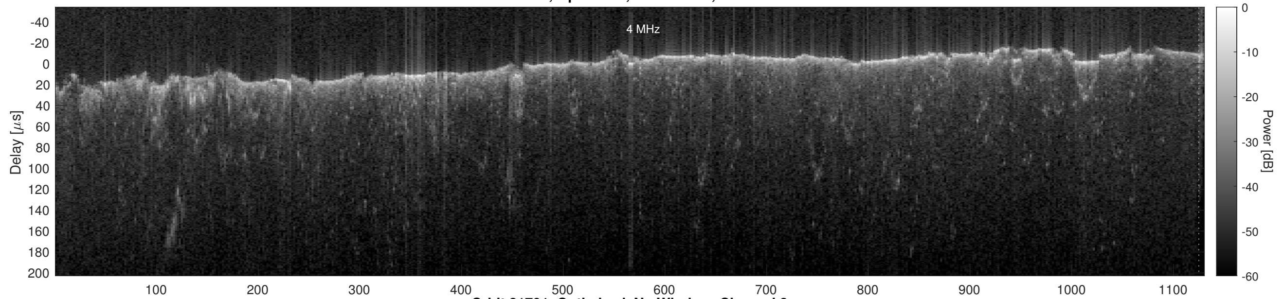
Orbit 21791, Optimized, No Window, Channel 2
