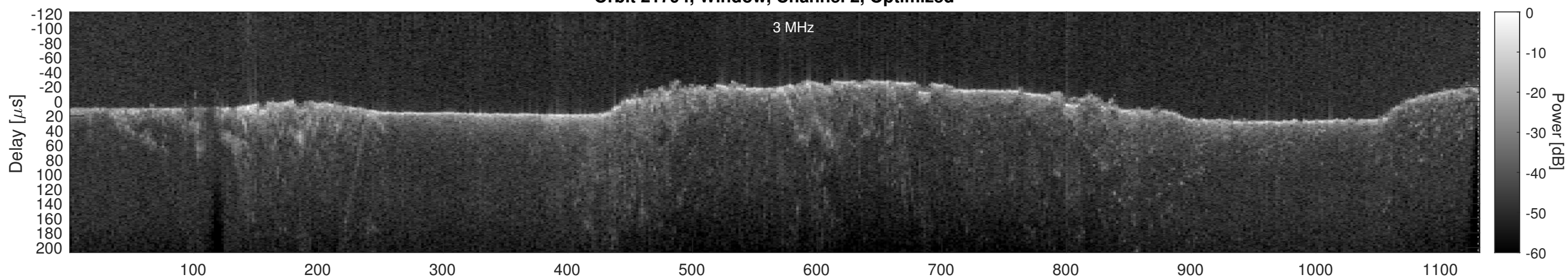
Orbit 21794, Cluttergram
