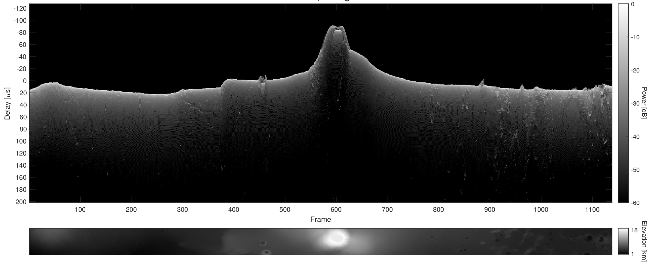
Orbit 21796, Cluttergram
