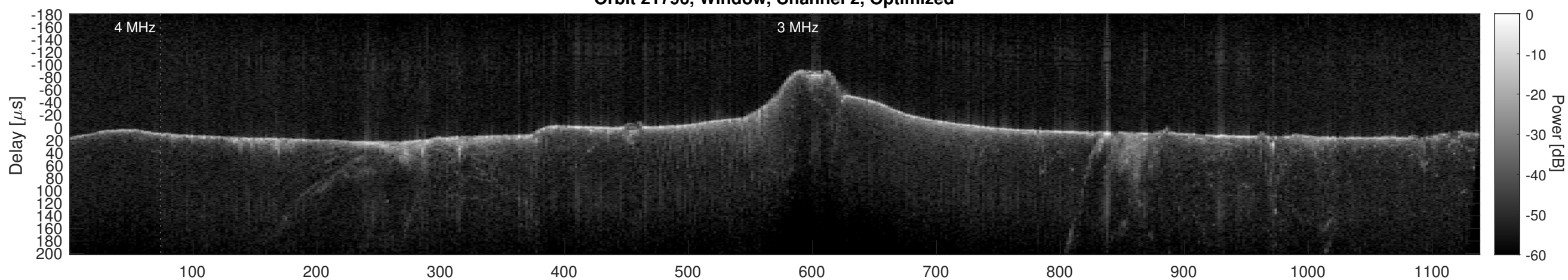
Orbit 21796, Cluttergram
