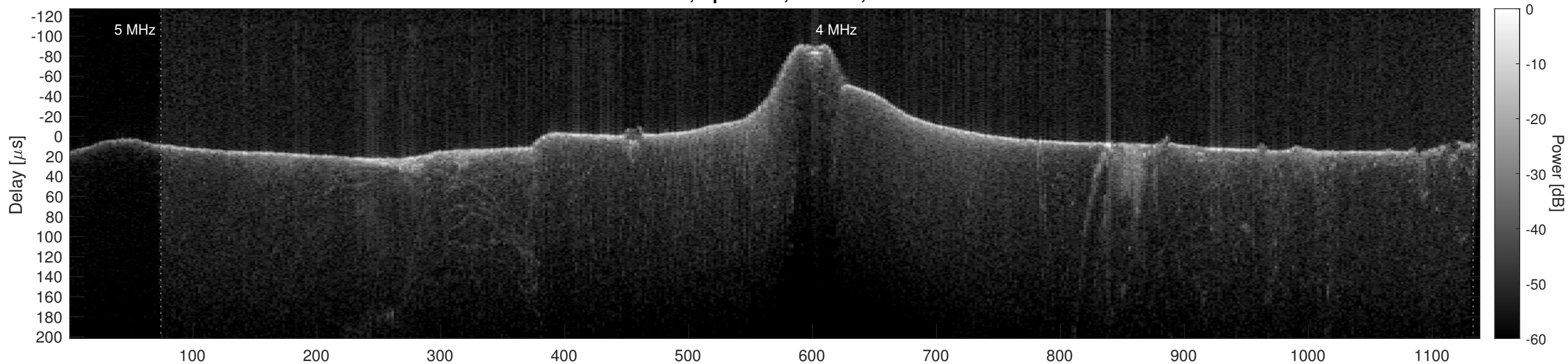
Orbit 21796, Optimized, Window, Channel 2
