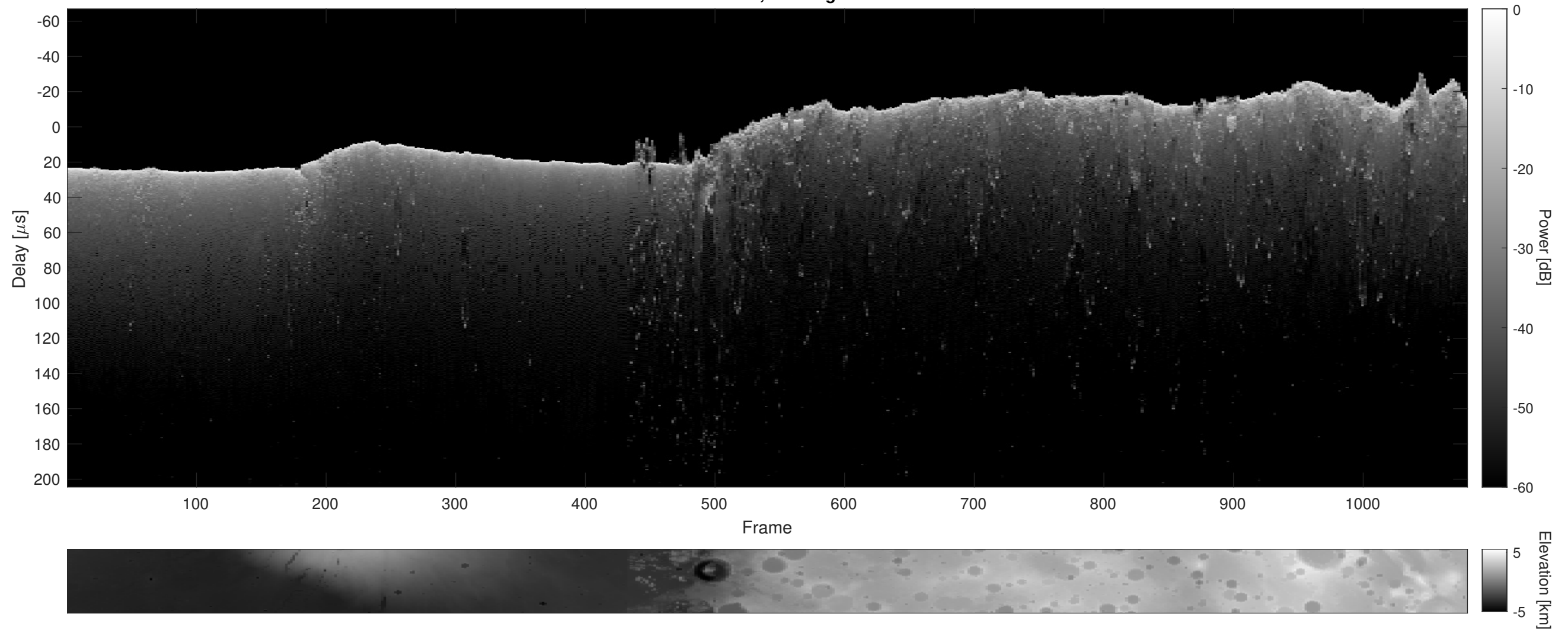
Orbit 21797, Cluttergram
