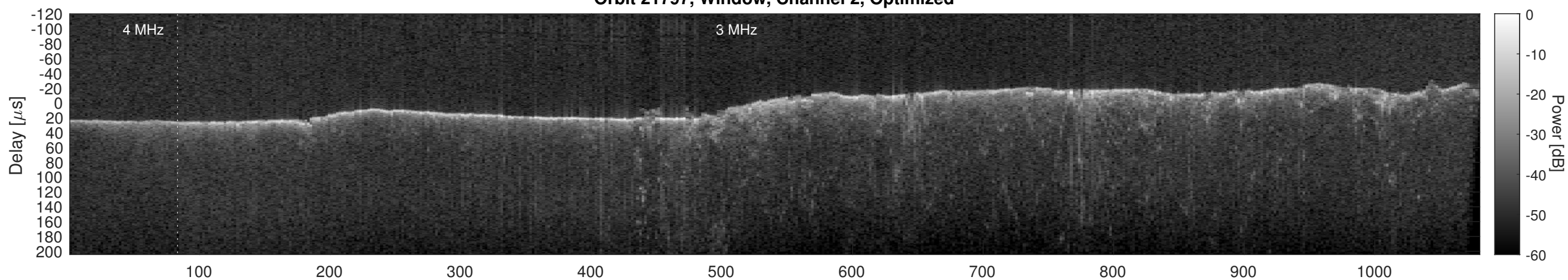
Orbit 21797, Cluttergram
