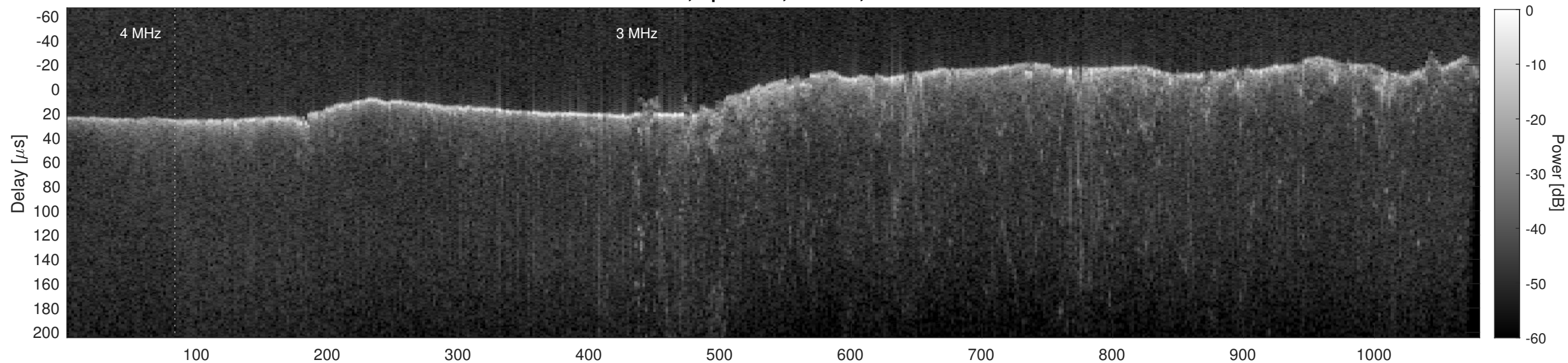
Orbit 21797, Cluttergram
