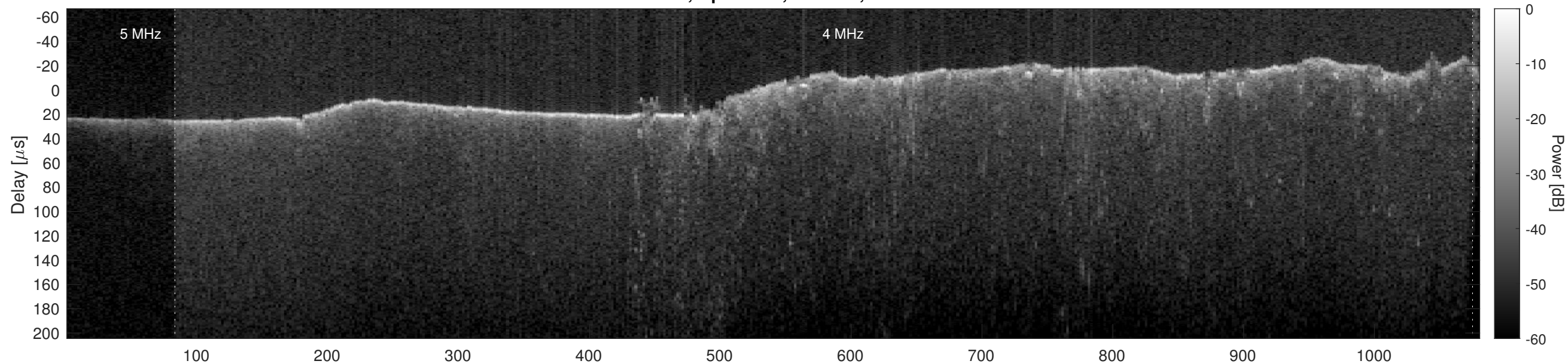
Orbit 21797, Optimized, Window, Channel 2
