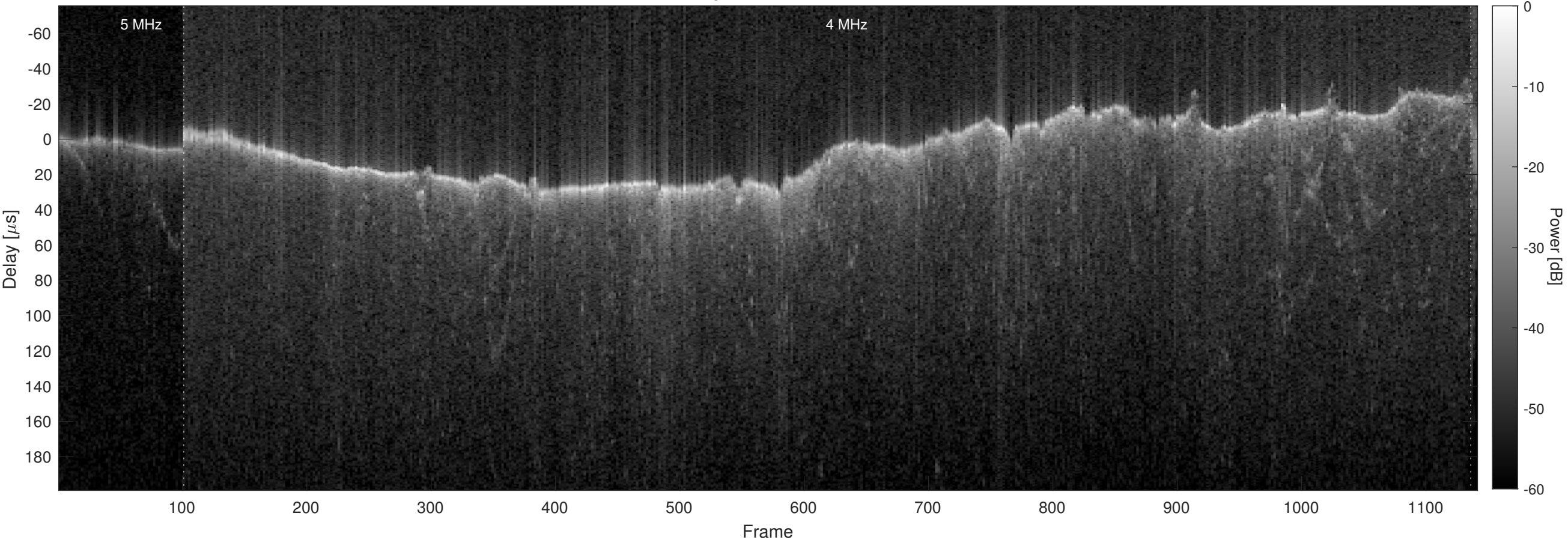
Orbit 21800, Chapman, No Window, Channel 2
