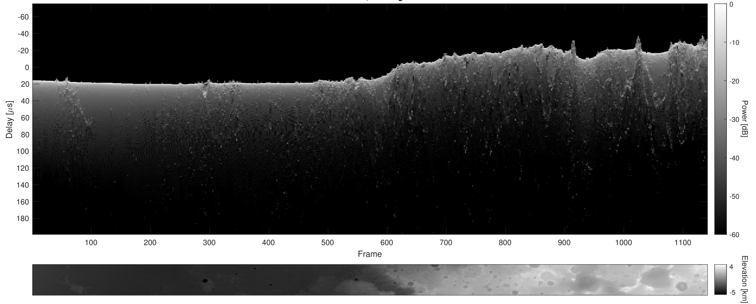
Orbit 21800, Cluttergram
