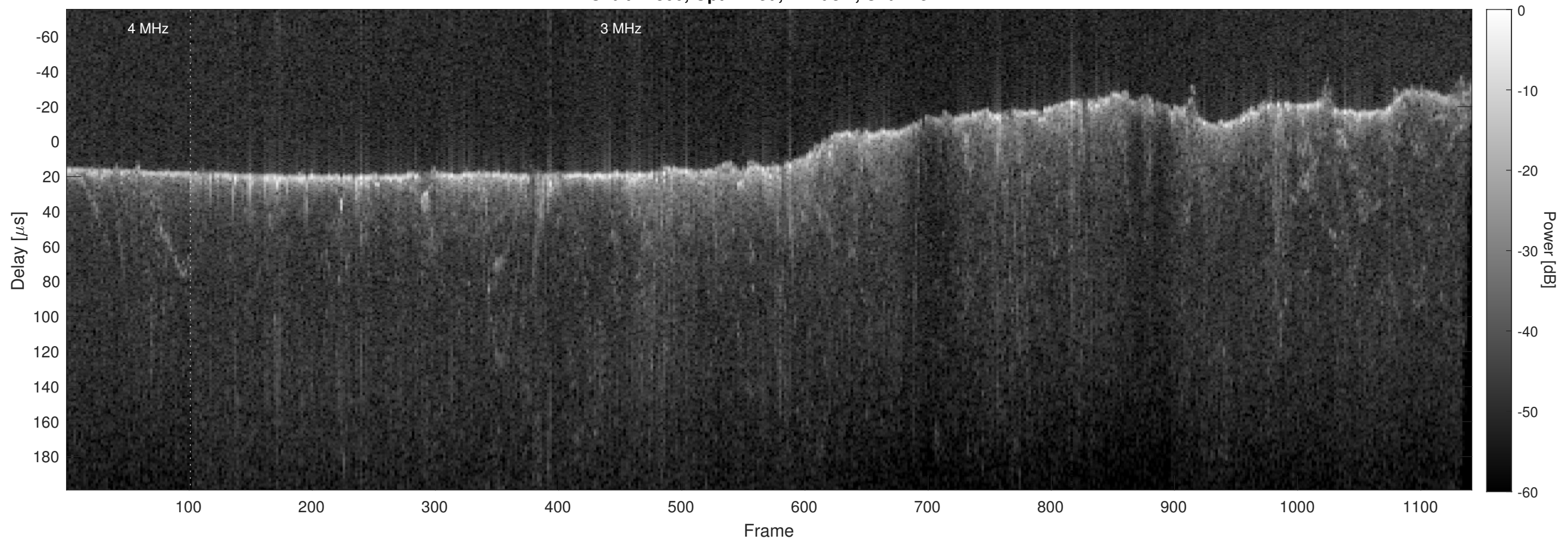
Orbit 21800, Optimized, Window, Channel 2
