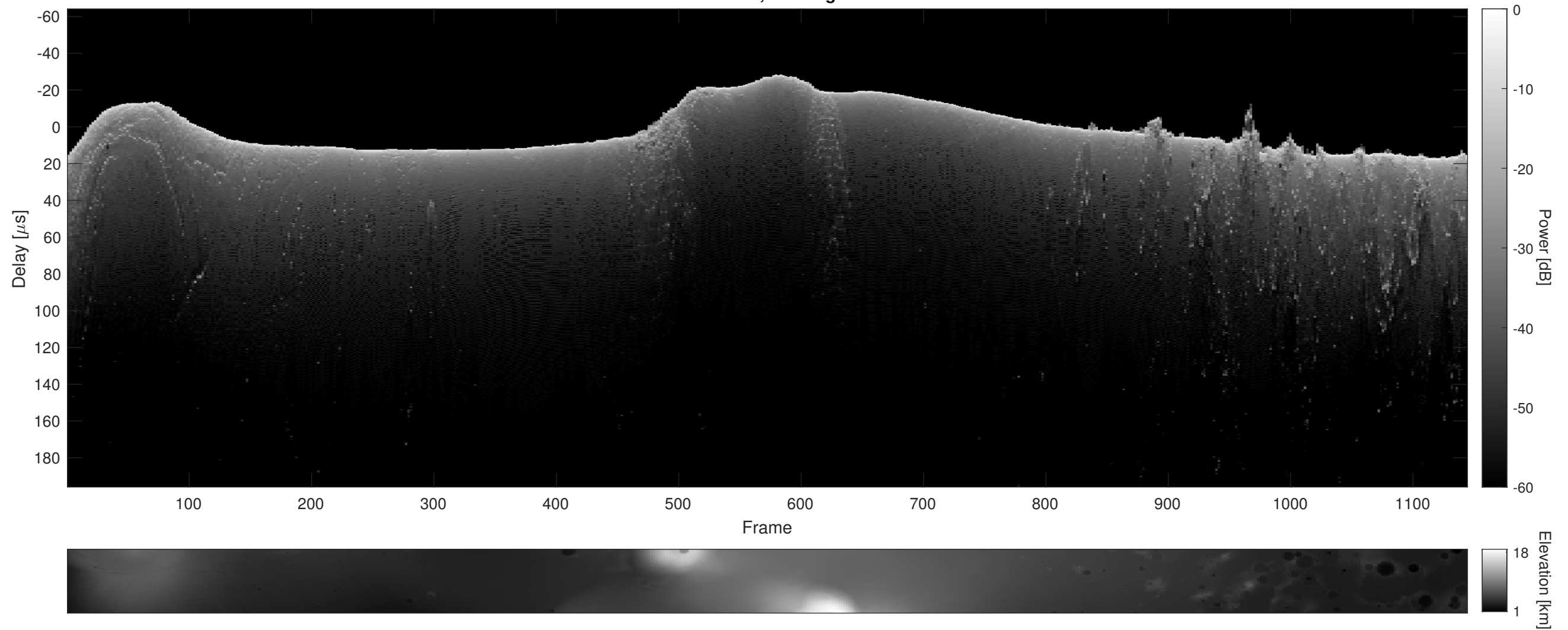
Orbit 21803, Cluttergram
