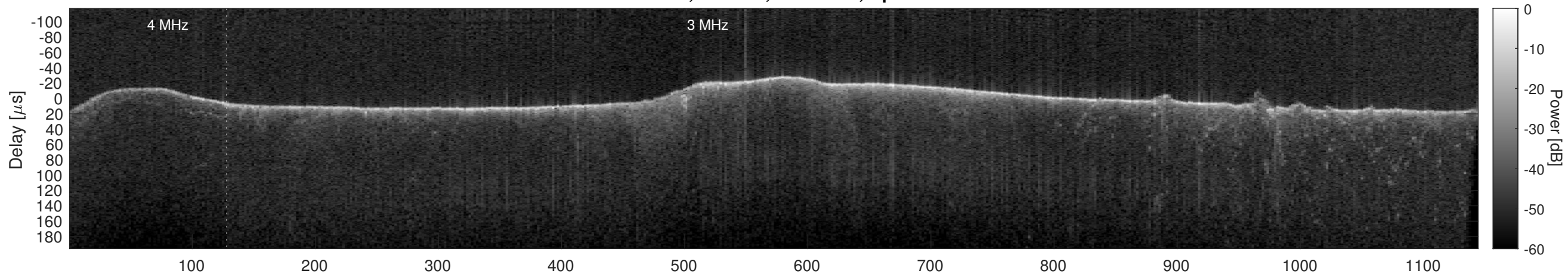
Orbit 21803, Cluttergram
