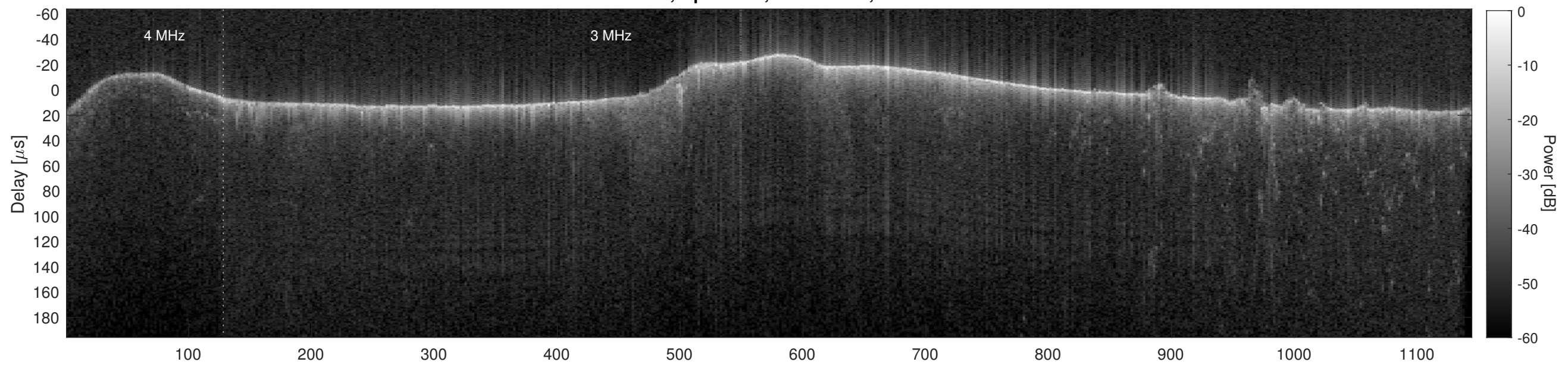
Orbit 21803, Cluttergram
