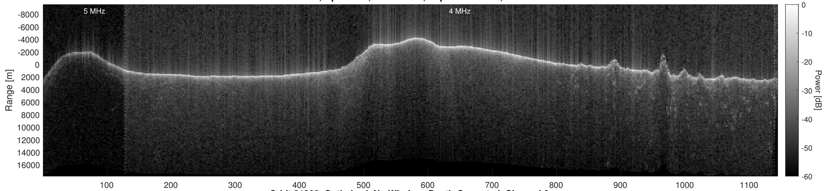
Orbit 21803, Optimized, No Window, Depth-Corrected, Channel 2
