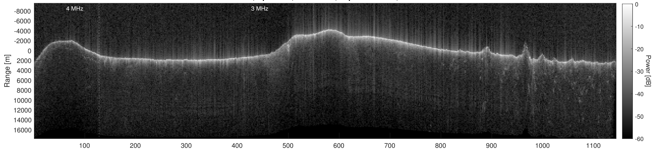
Orbit 21803, Depth-Corrected Cluttergram
