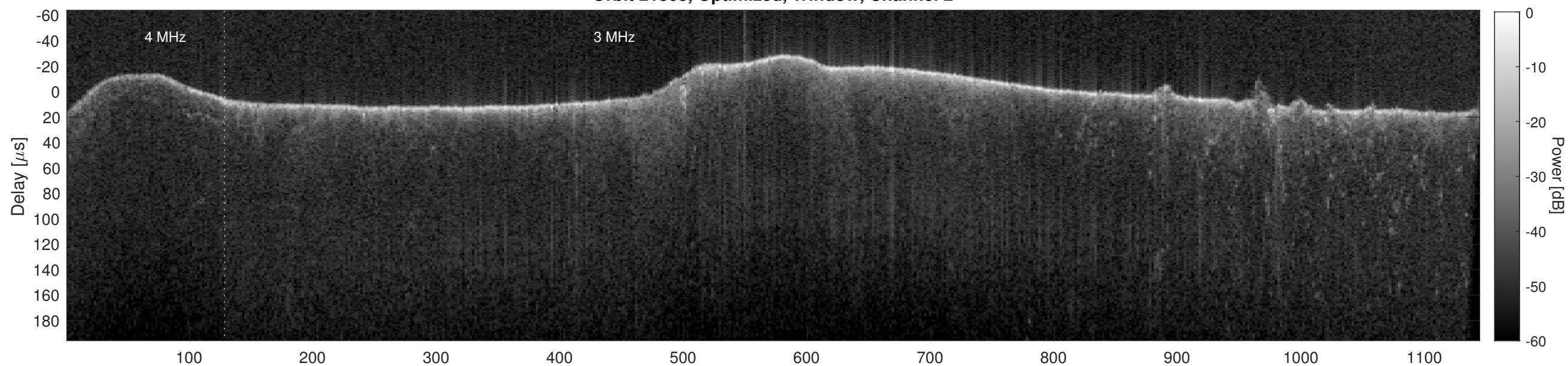
Orbit 21803, Cluttergram
