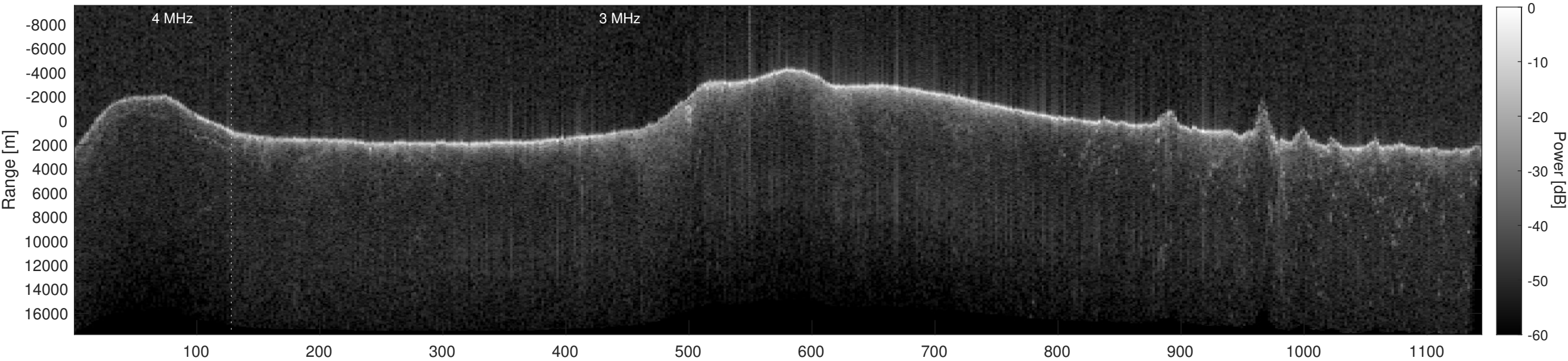
Orbit 21803, Depth-Corrected Cluttergram
