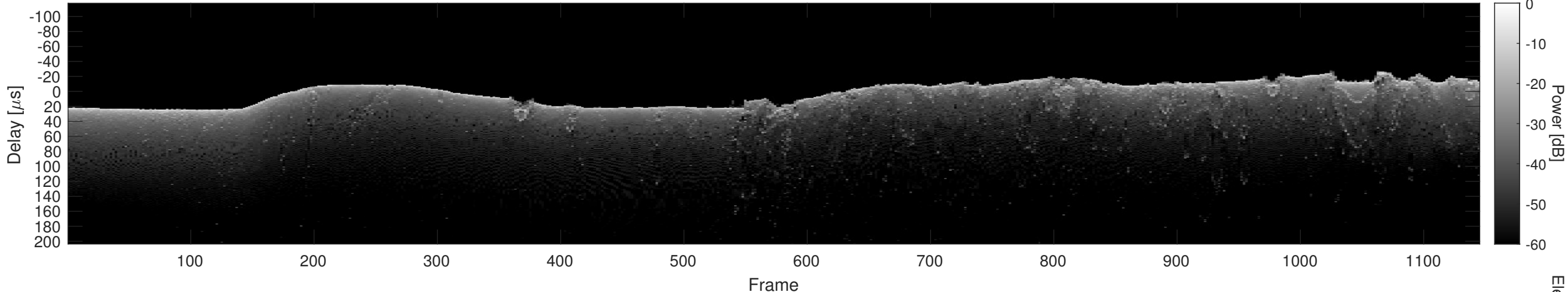
Orbit 21804, Cluttergram
