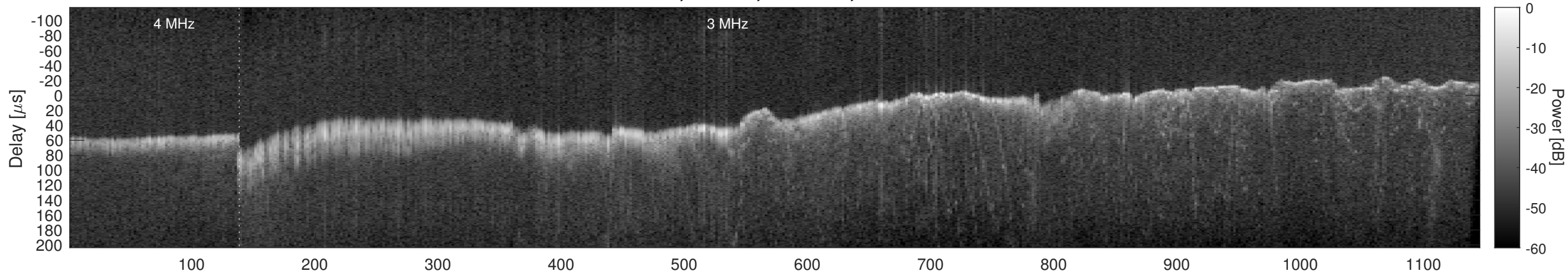
Orbit 21804, Window, Channel 2, Chapman
