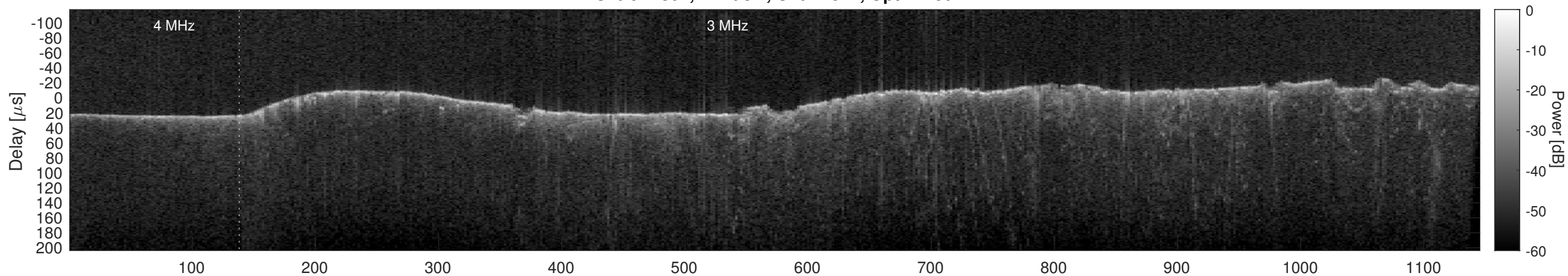
Orbit 21804, Cluttergram
