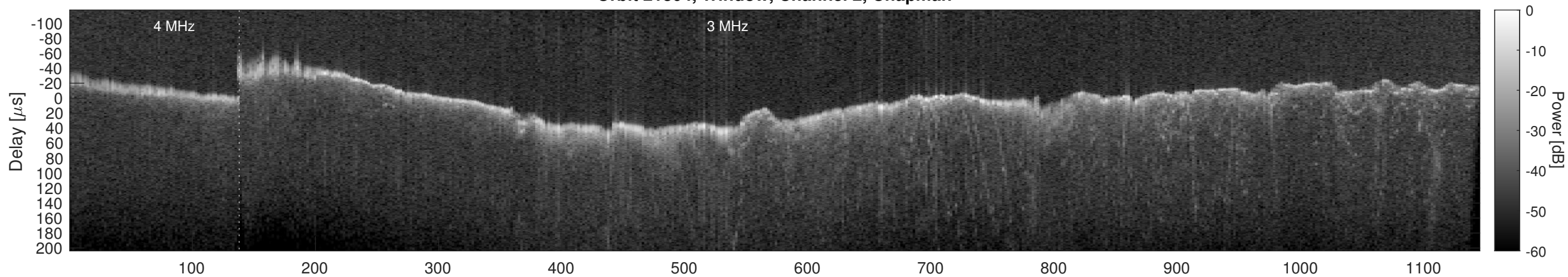
Orbit 21804, Window, Channel 2, Optimized
