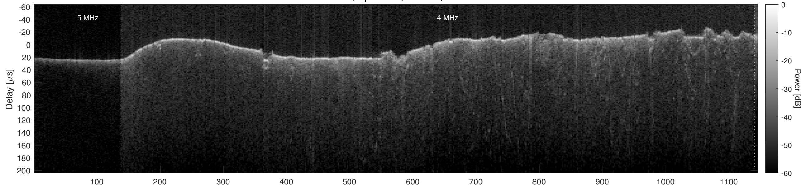
Orbit 21804, Optimized, Window, Channel 2
