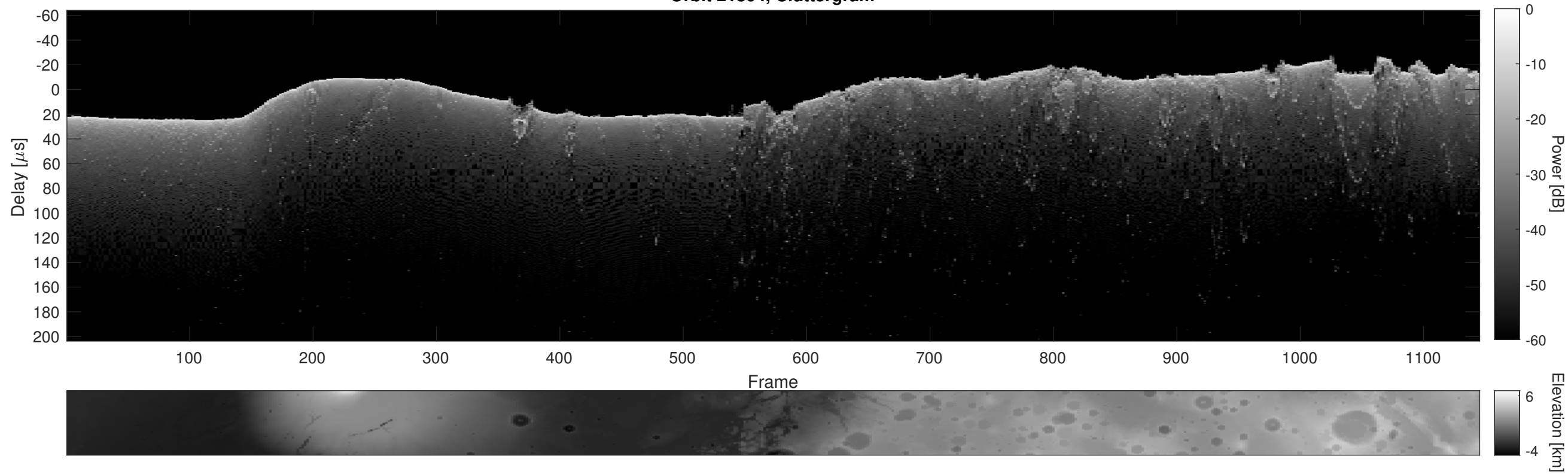
Orbit 21804, Cluttergram
