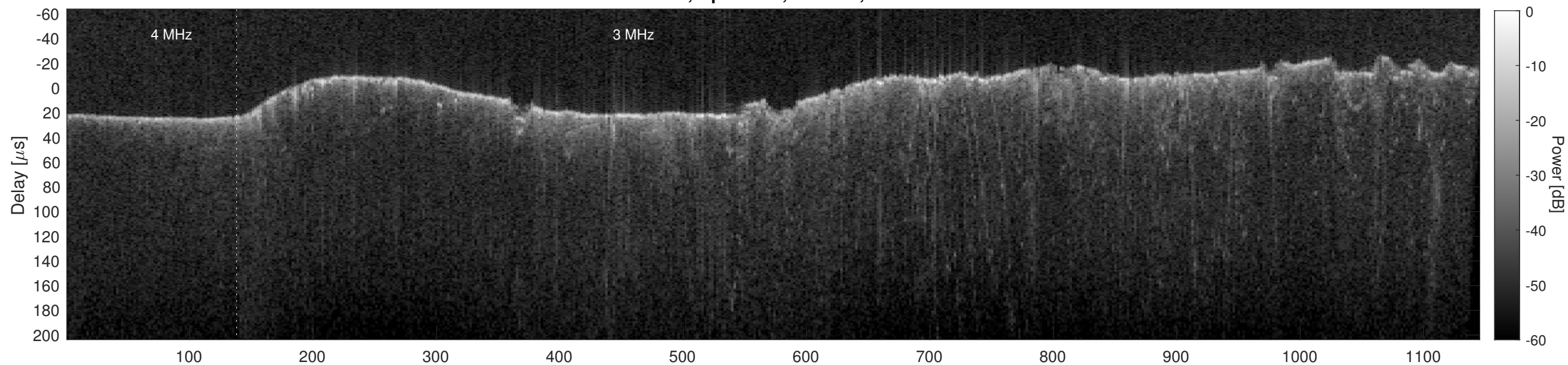
Orbit 21804, Cluttergram
