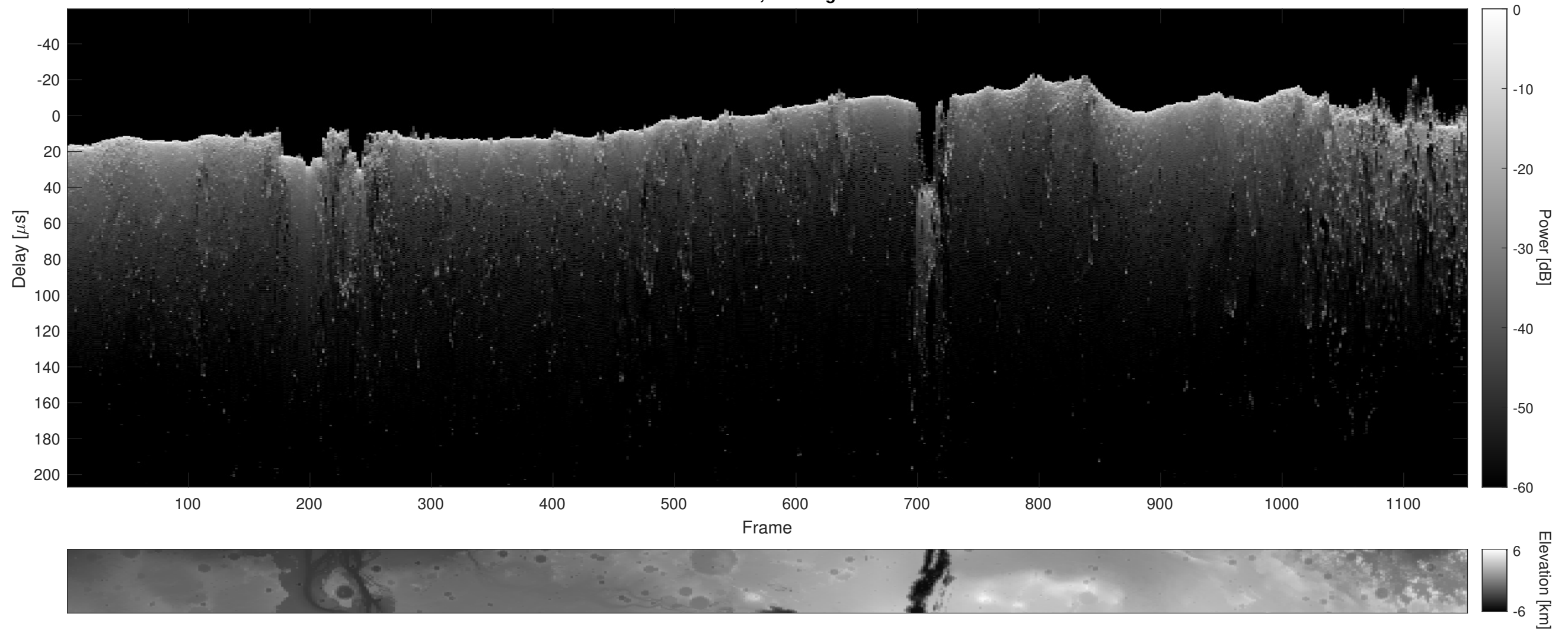
Orbit 21813, Cluttergram
