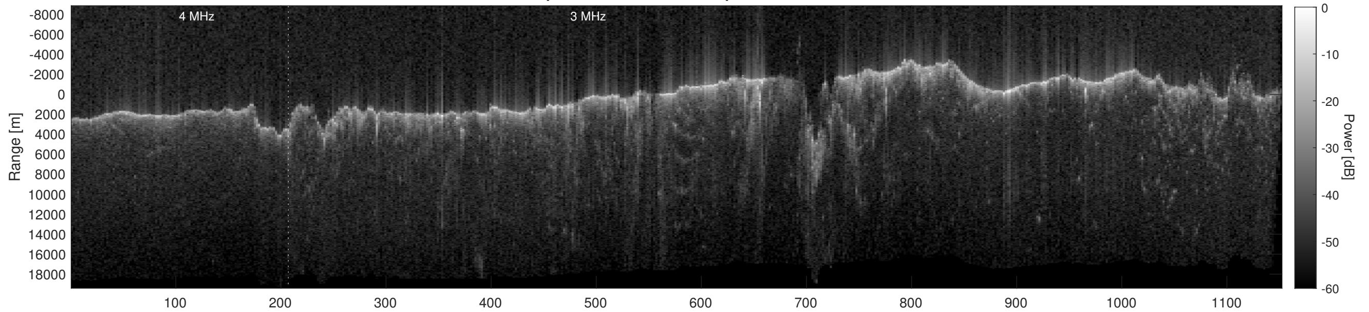
Orbit 21813, Depth-Corrected Cluttergram
