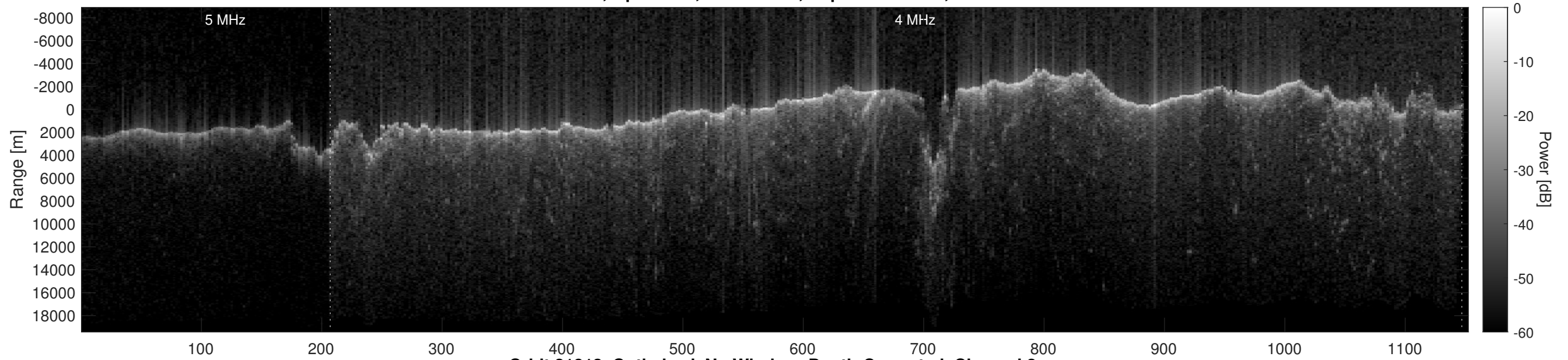
Orbit 21813, Optimized, No Window, Depth-Corrected, Channel 2
