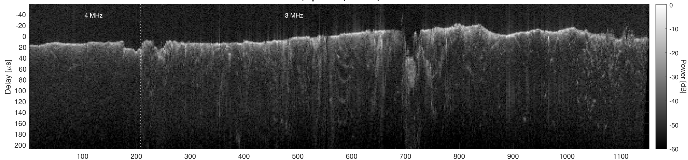
Orbit 21813, Cluttergram
