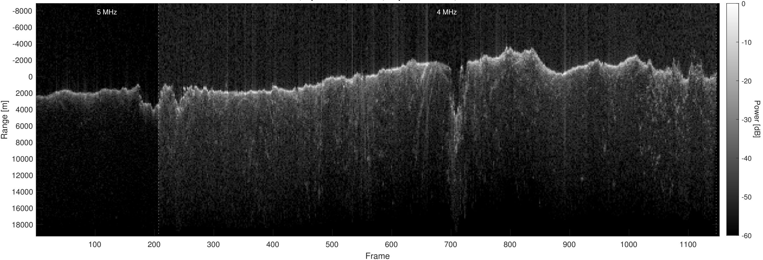
Orbit 21813, Optimized, Window, Depth-Corrected, Channel 2
