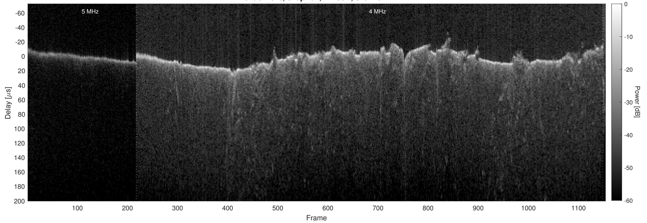
Orbit 21815, Chapman, Window, Channel 2
