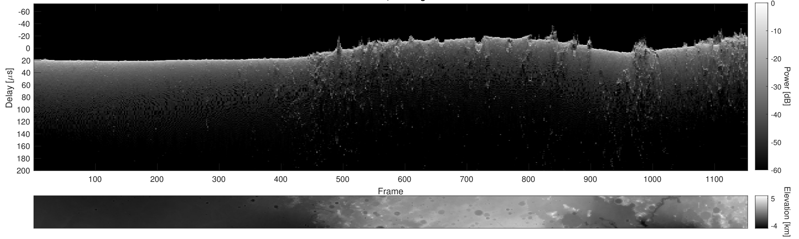
Orbit 21815, Cluttergram
