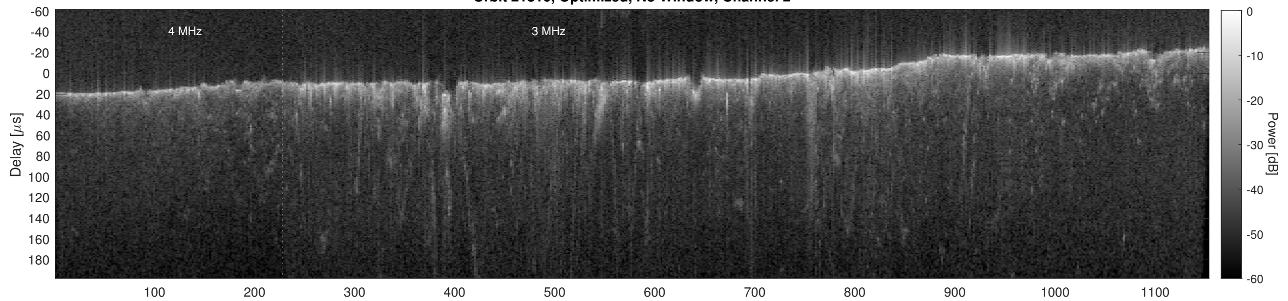
Orbit 21816, Cluttergram
