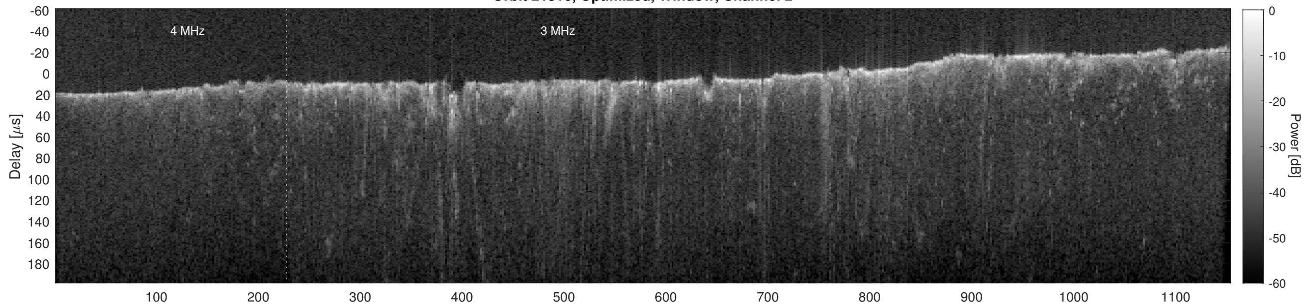
Orbit 21816, Cluttergram
