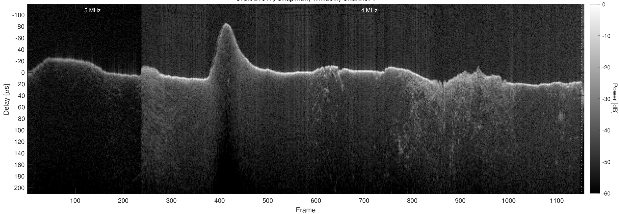
Orbit 21817, Chapman, Window, Channel 2
