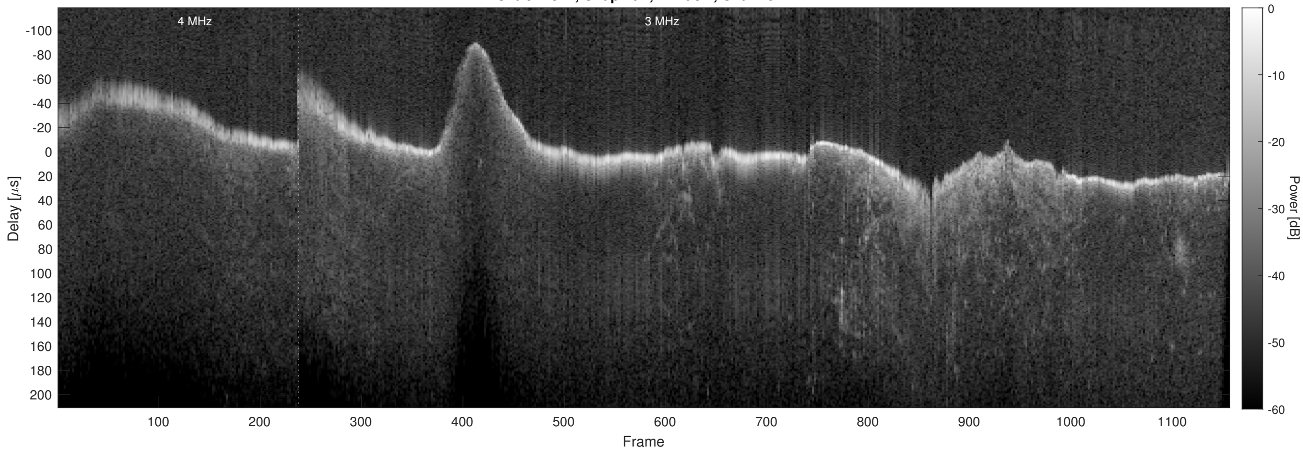
Orbit 21817, Chapman, Window, Channel 2
