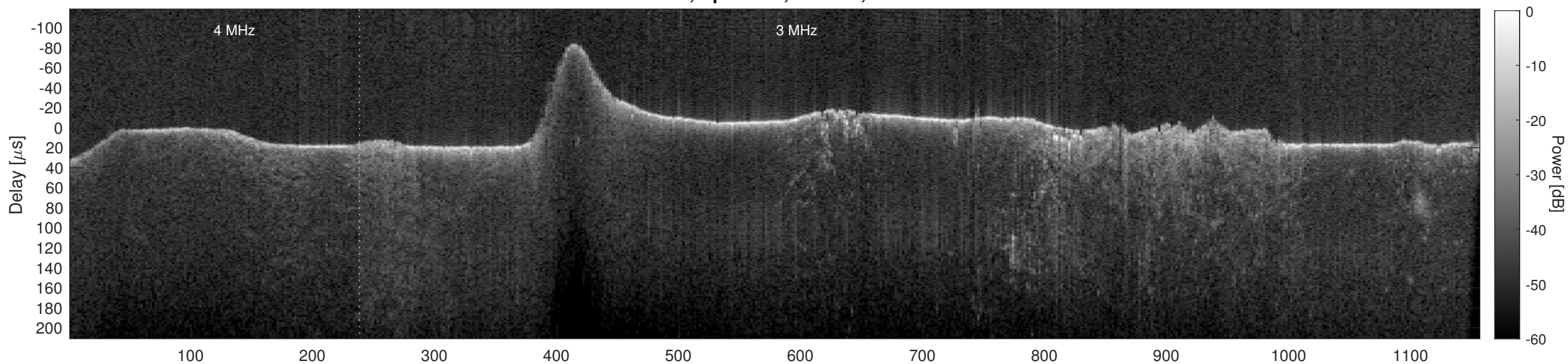
Orbit 21817, Cluttergram
