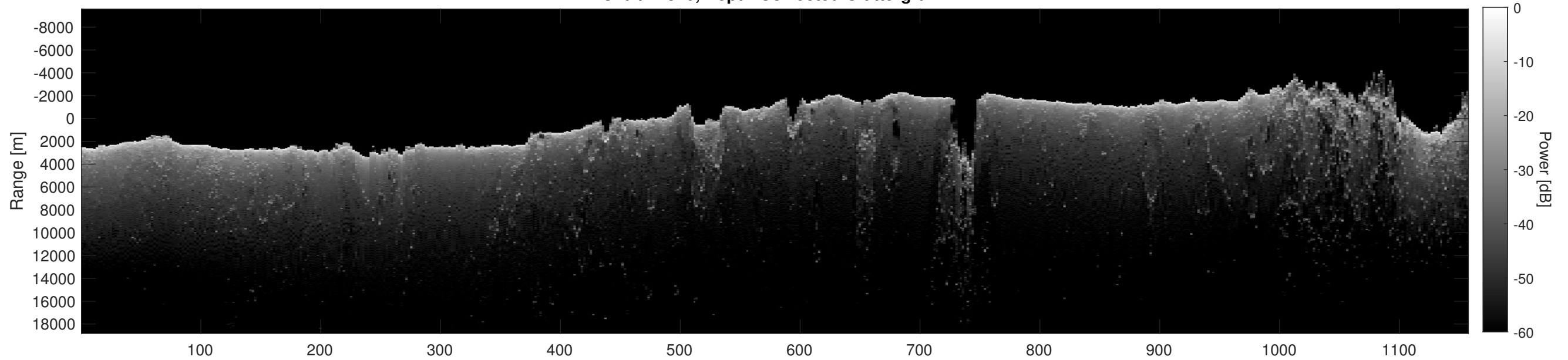
Orbit 21820, Depth-Corrected Cluttergram
