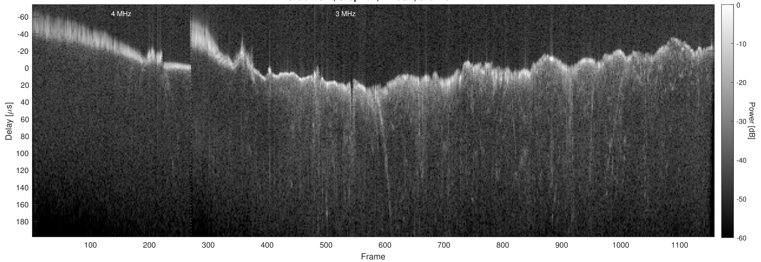
Orbit 21821, Chapman, Window, Channel 2
