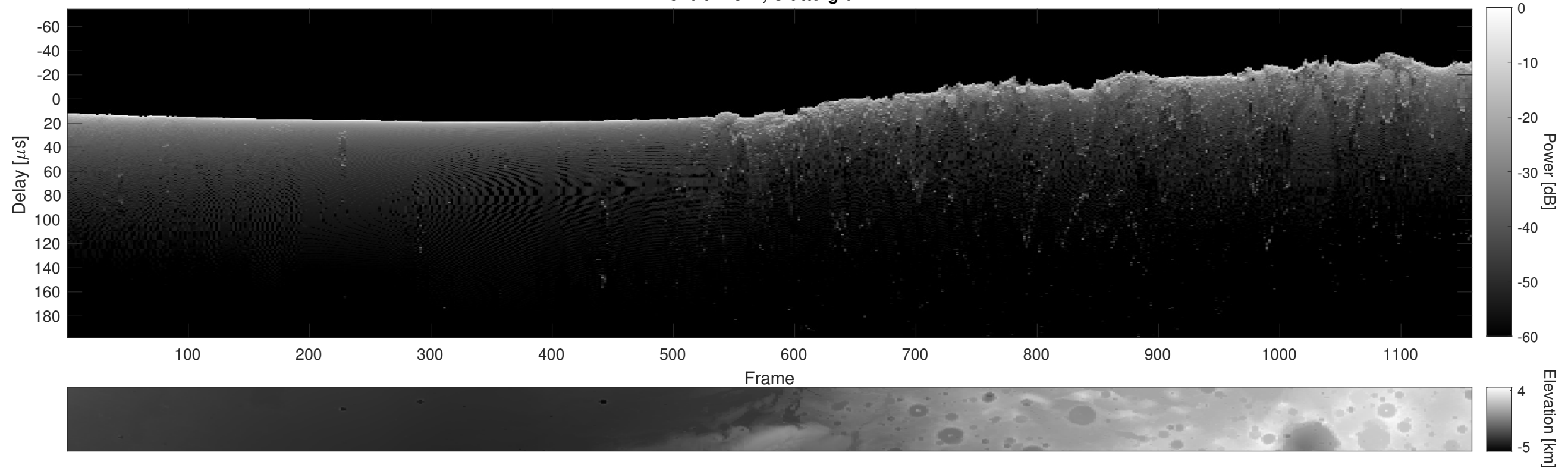
Orbit 21821, Cluttergram
