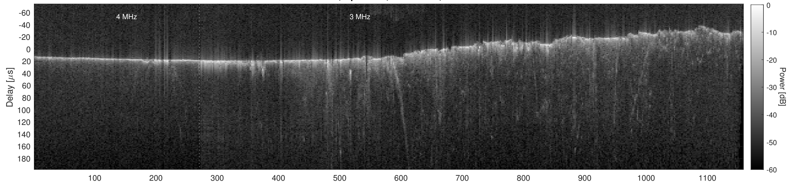
Orbit 21821, Cluttergram
