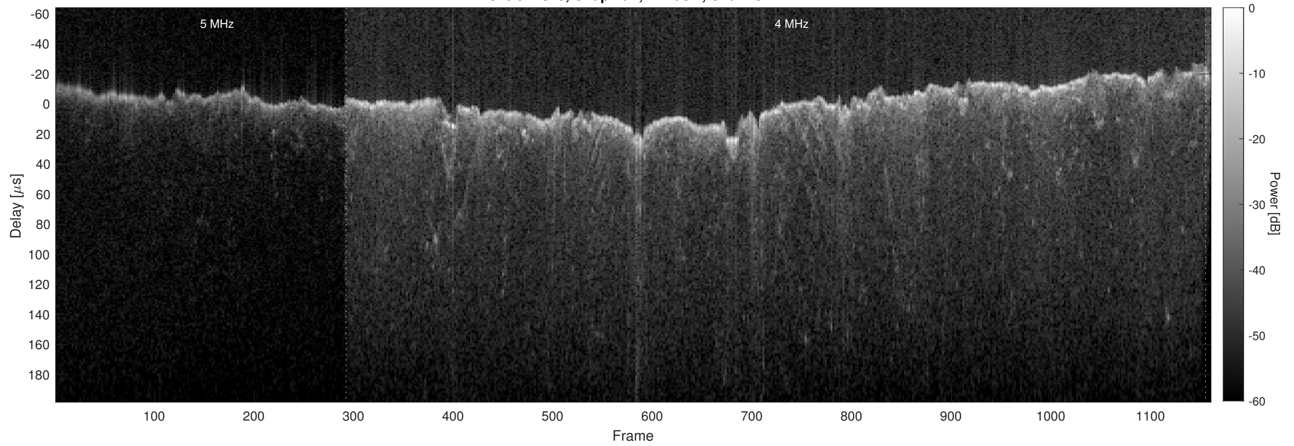
Orbit 21823, Chapman, Window, Channel 2
