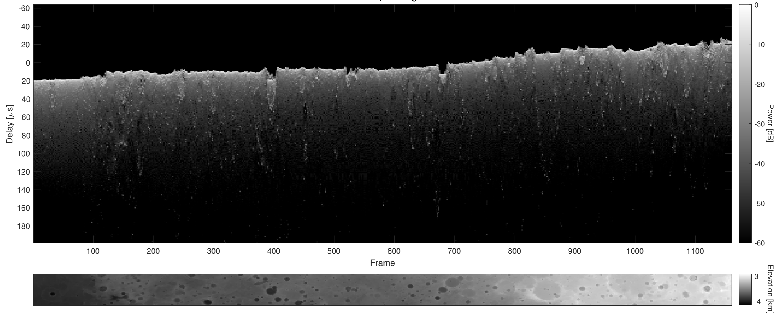
Orbit 21823, Cluttergram
