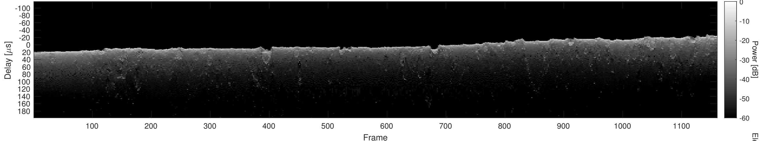
Orbit 21823, Cluttergram
