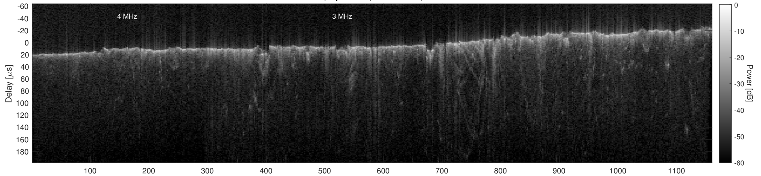
Orbit 21823, Cluttergram
