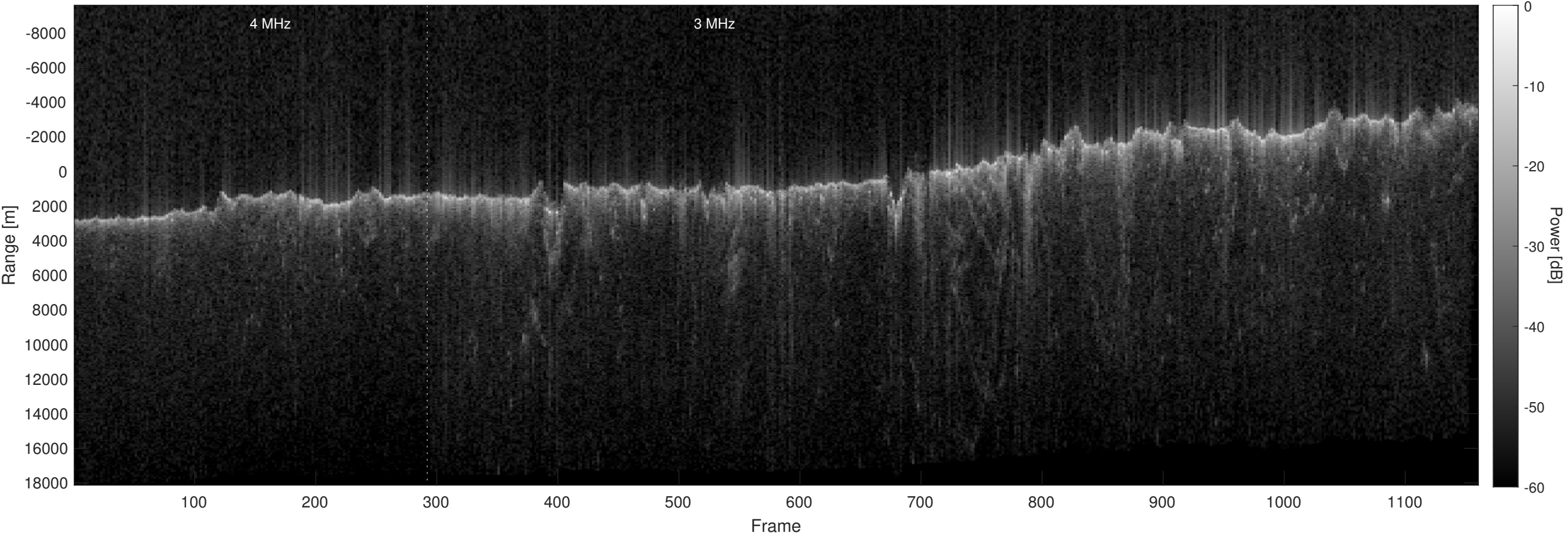
Orbit 21823, Optimized, No Window, Depth-Corrected, Channel 2
