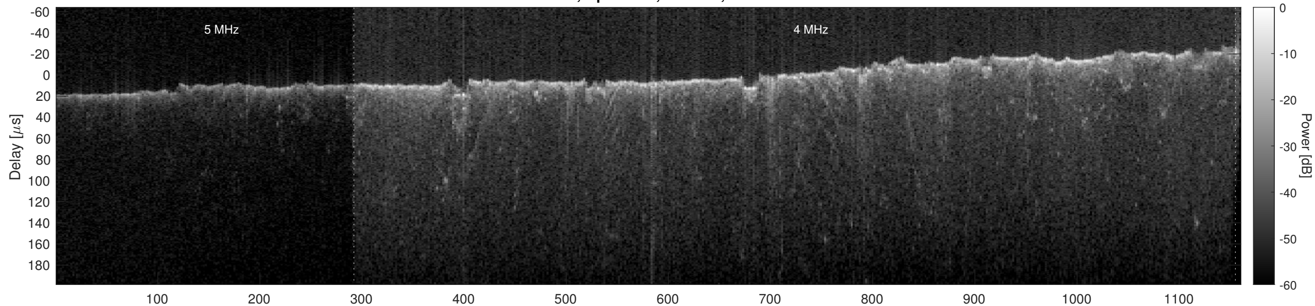
Orbit 21823, Optimized, Window, Channel 2
