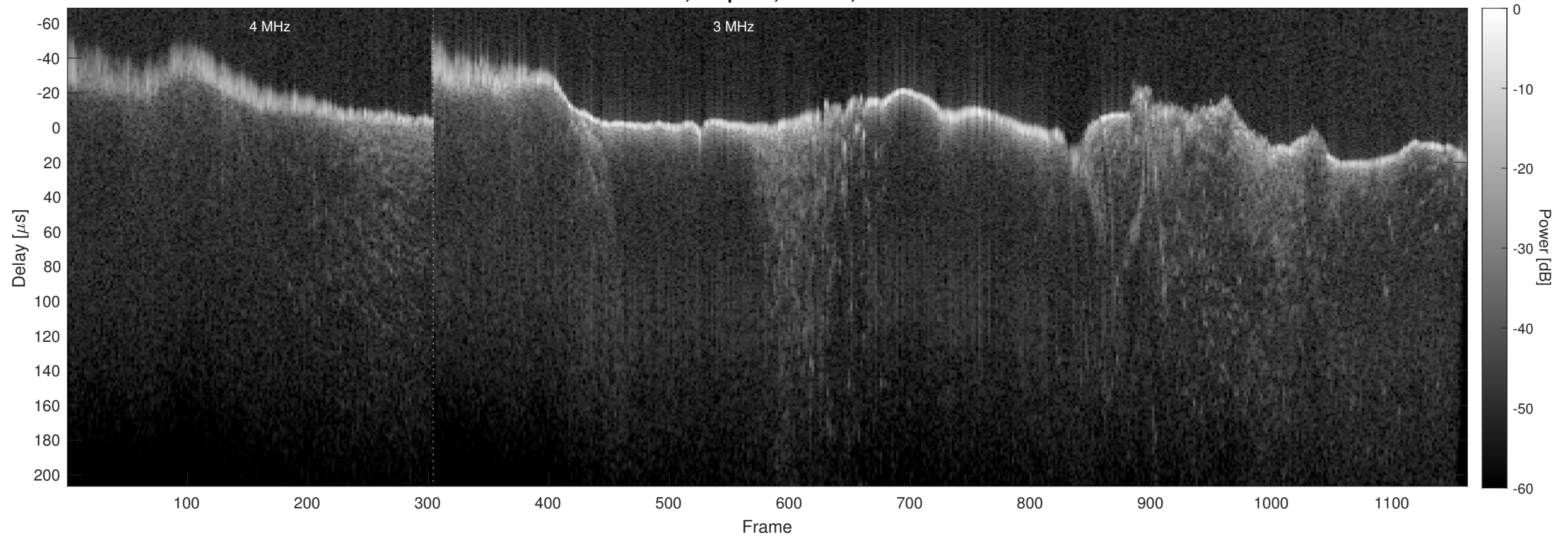
Orbit 21824, Chapman, Window, Channel 2
