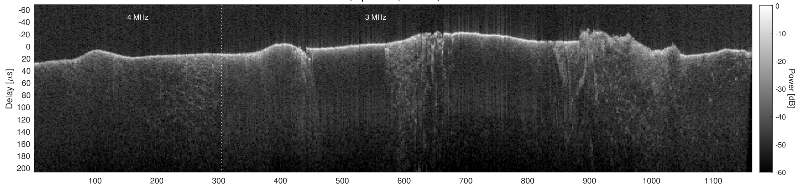
Orbit 21824, Cluttergram
