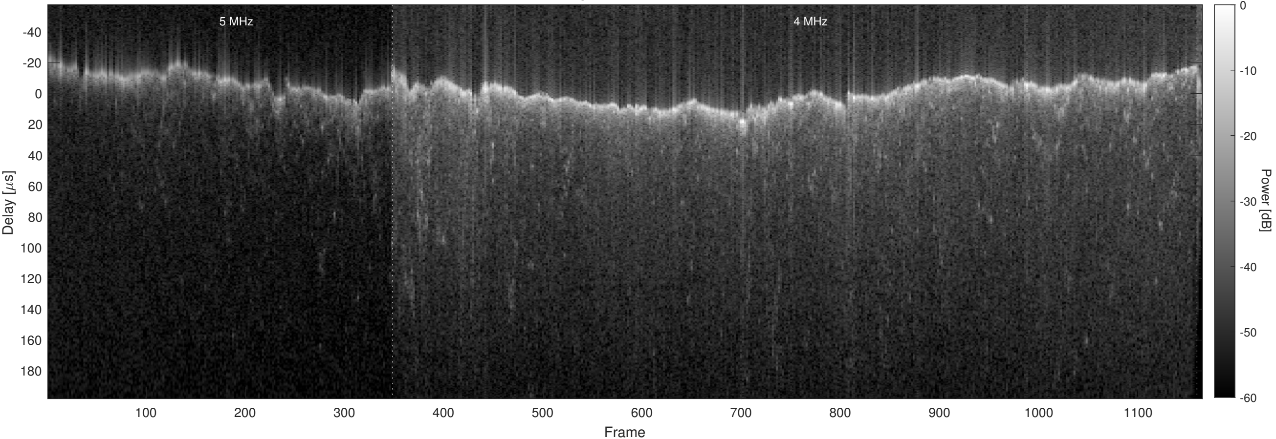
Orbit 21830, Chapman, No Window, Channel 2
