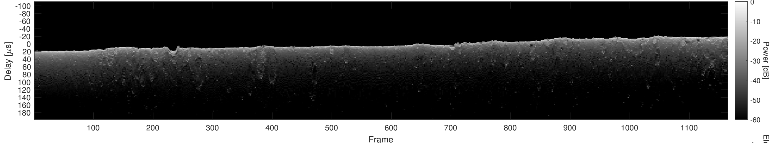
Orbit 21830, Cluttergram
